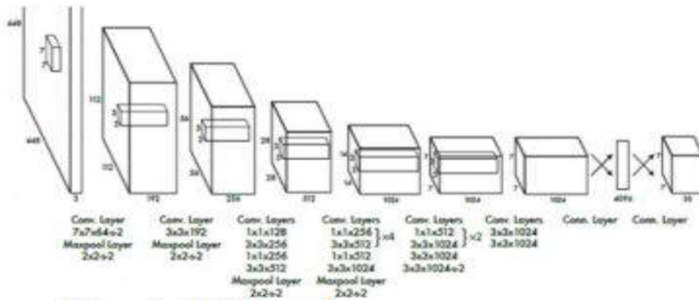
Figure6 : YOLO architecture
