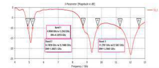
Fig.4: The bandwidth graph
