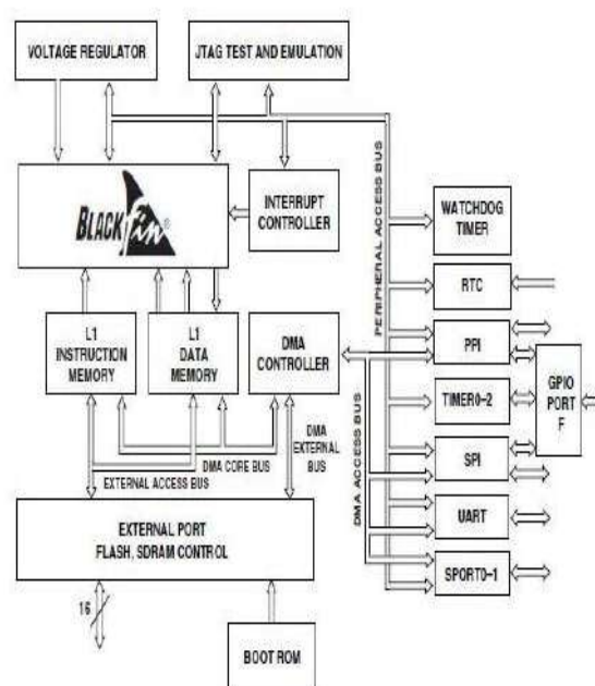
Figure 1.1 Blackfin Processor Architecture
