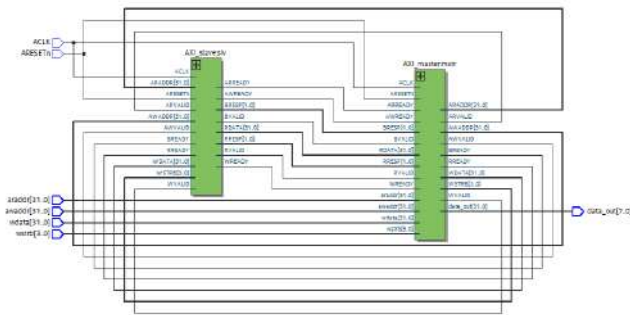
Fig. 3. RTL Design for AXI top.
