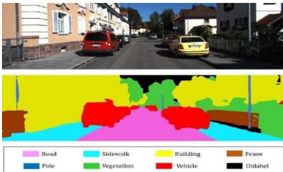
Fig 6: Image segmentation
