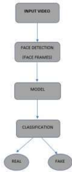
Fig. 3. Proposed Methodology
