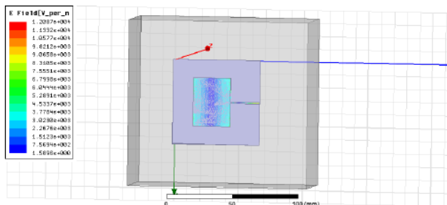
Fig.6(d) Electric Field distribution of rectangular microstrip antenna with polyster material
